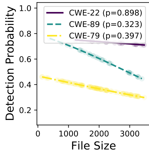
mixtral-8x7b
