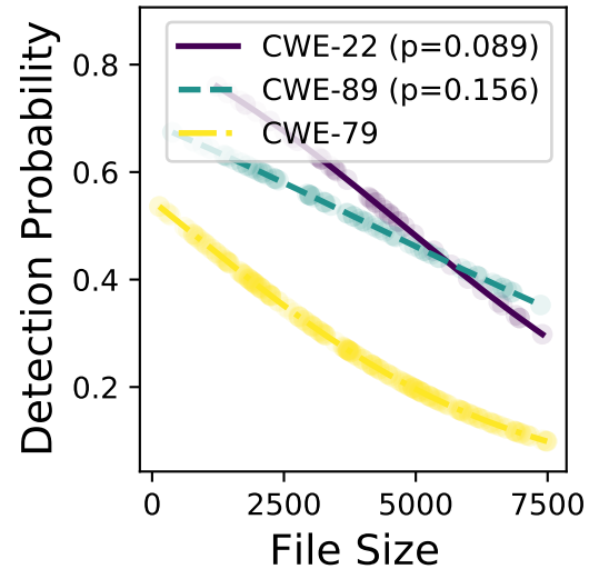
mixtral-8x7b
