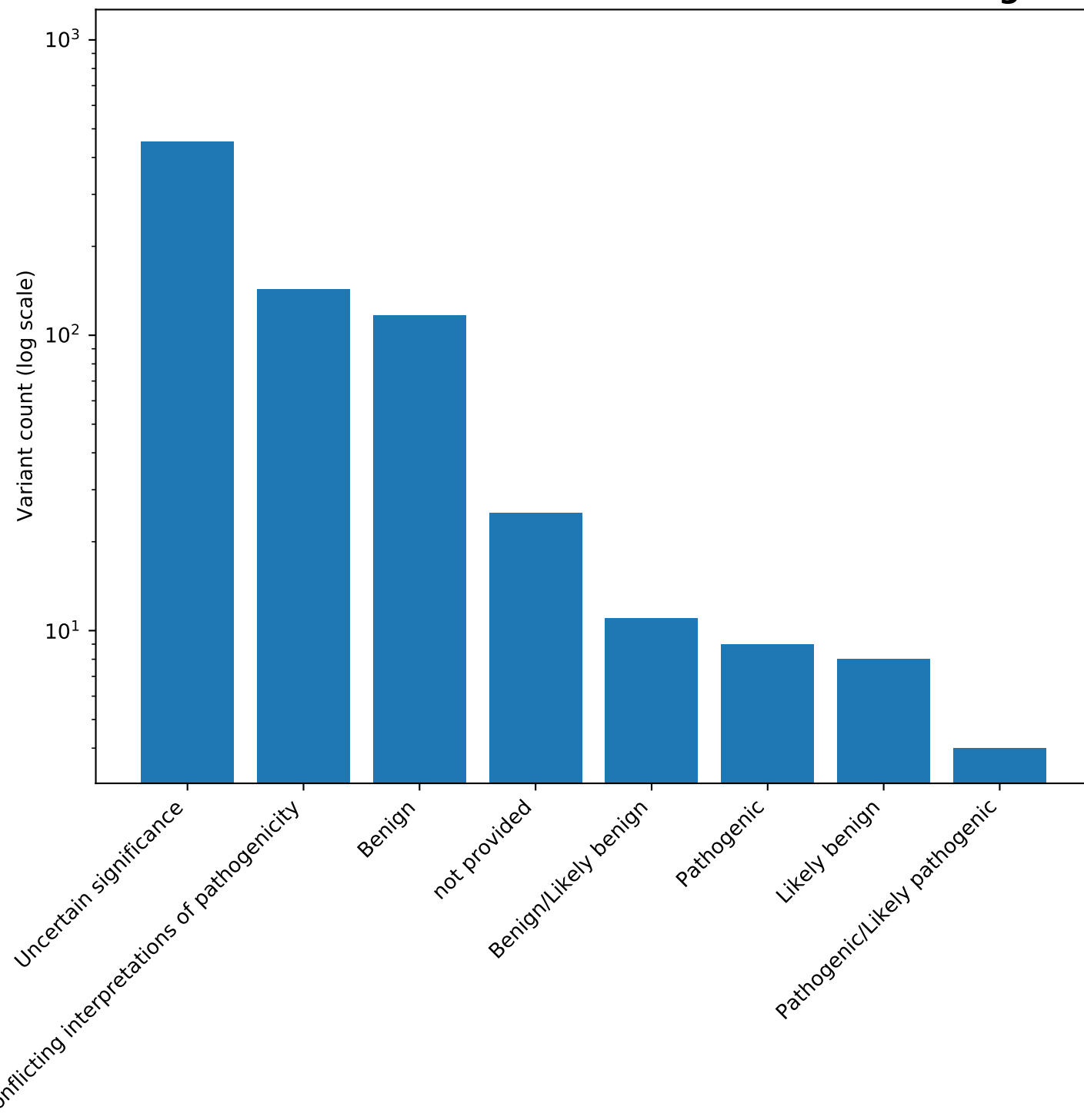
ClinVar annotations of missense variants in BRCA1 gene
