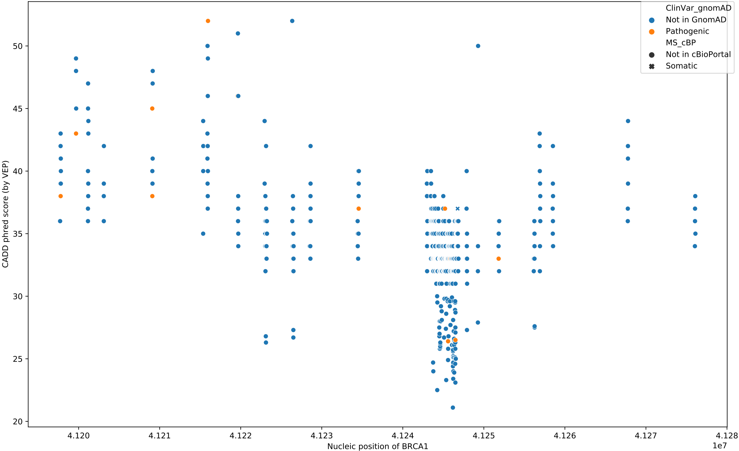
Stop Gained Variants in BRCA1 with ClinVar annotations of GnomAD
