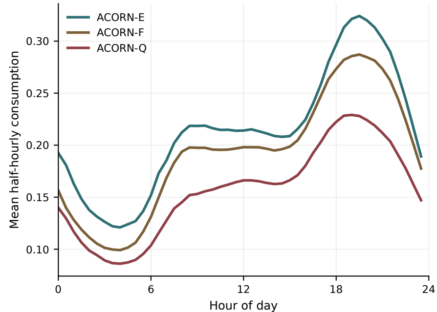
Typical half-hourly profile
