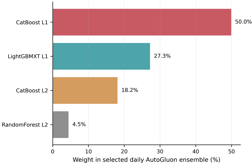
A AutoGluon daily: WeightedEnsemble_L3_FULL
