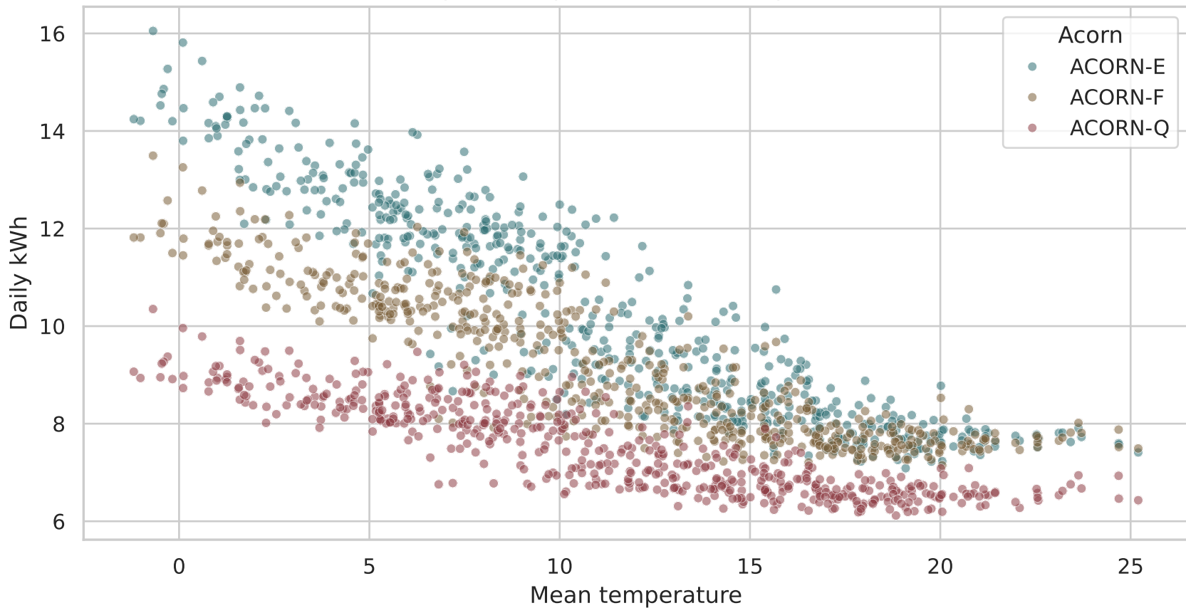
Daily consumption vs. mean temperature
