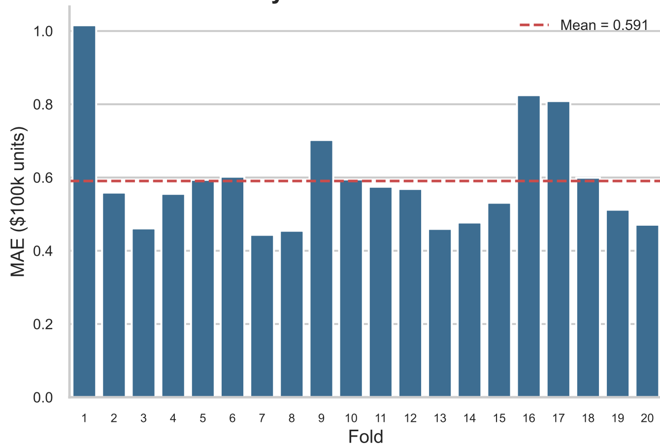
MAE by Cross-Validation Fold
