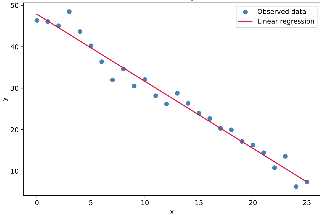
Dataset 1: Linear Regression Fit
