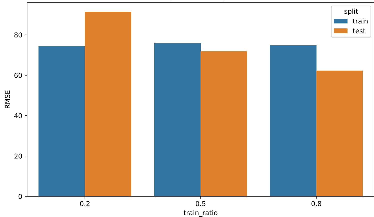
Ordered Splits: RMSE by Train Ratio
