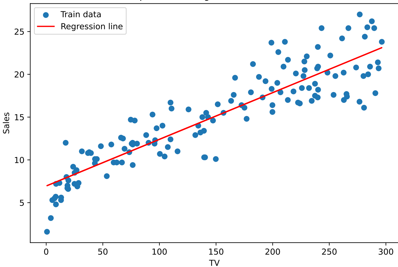
Simple Linear Regression: Sales vs TV
