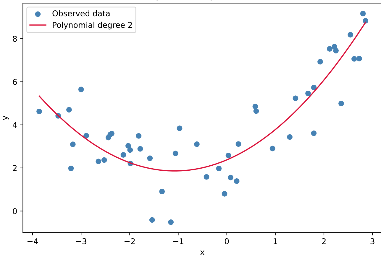
Polynomial Regression Fit
