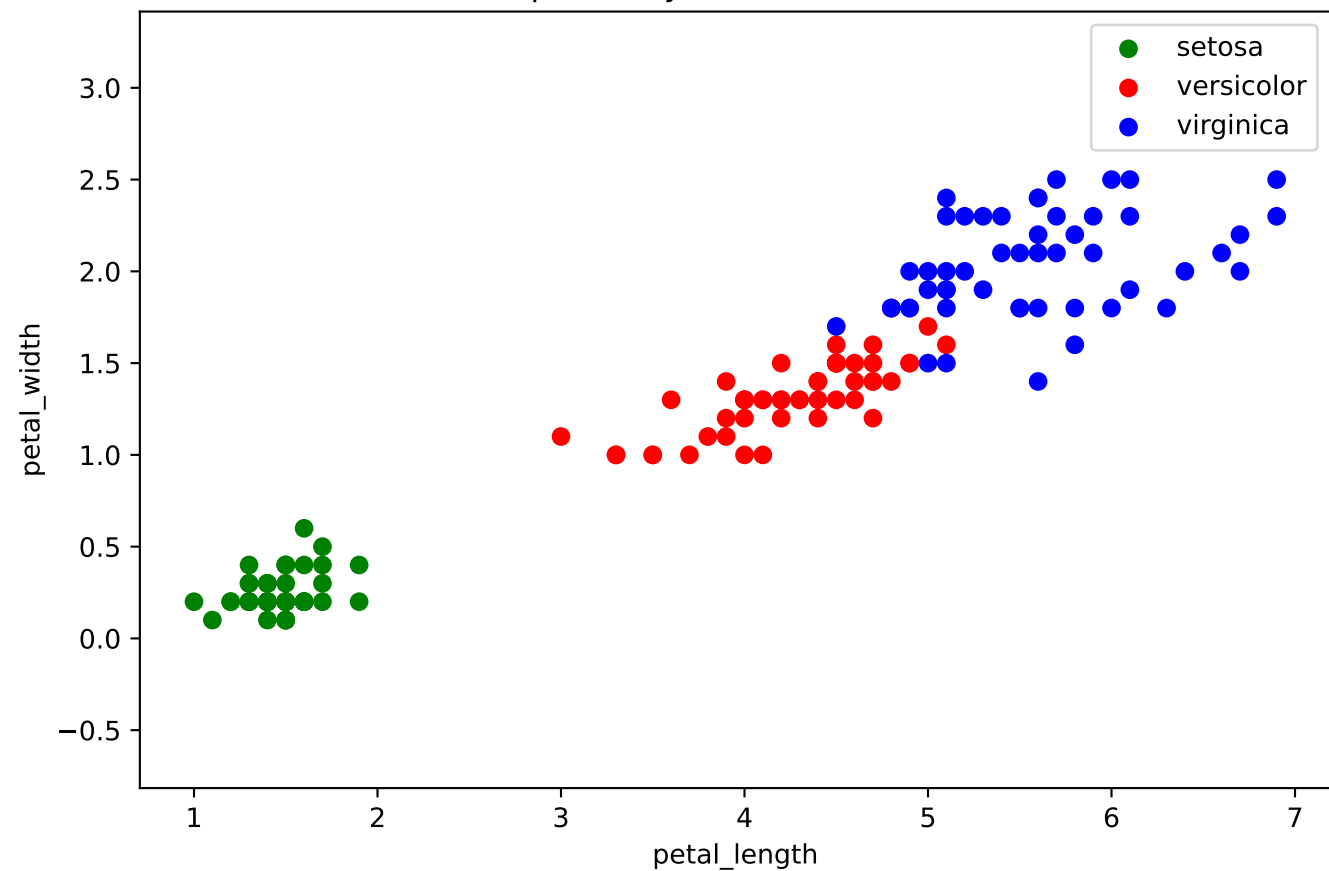
Iris Species by Petal Measurements
