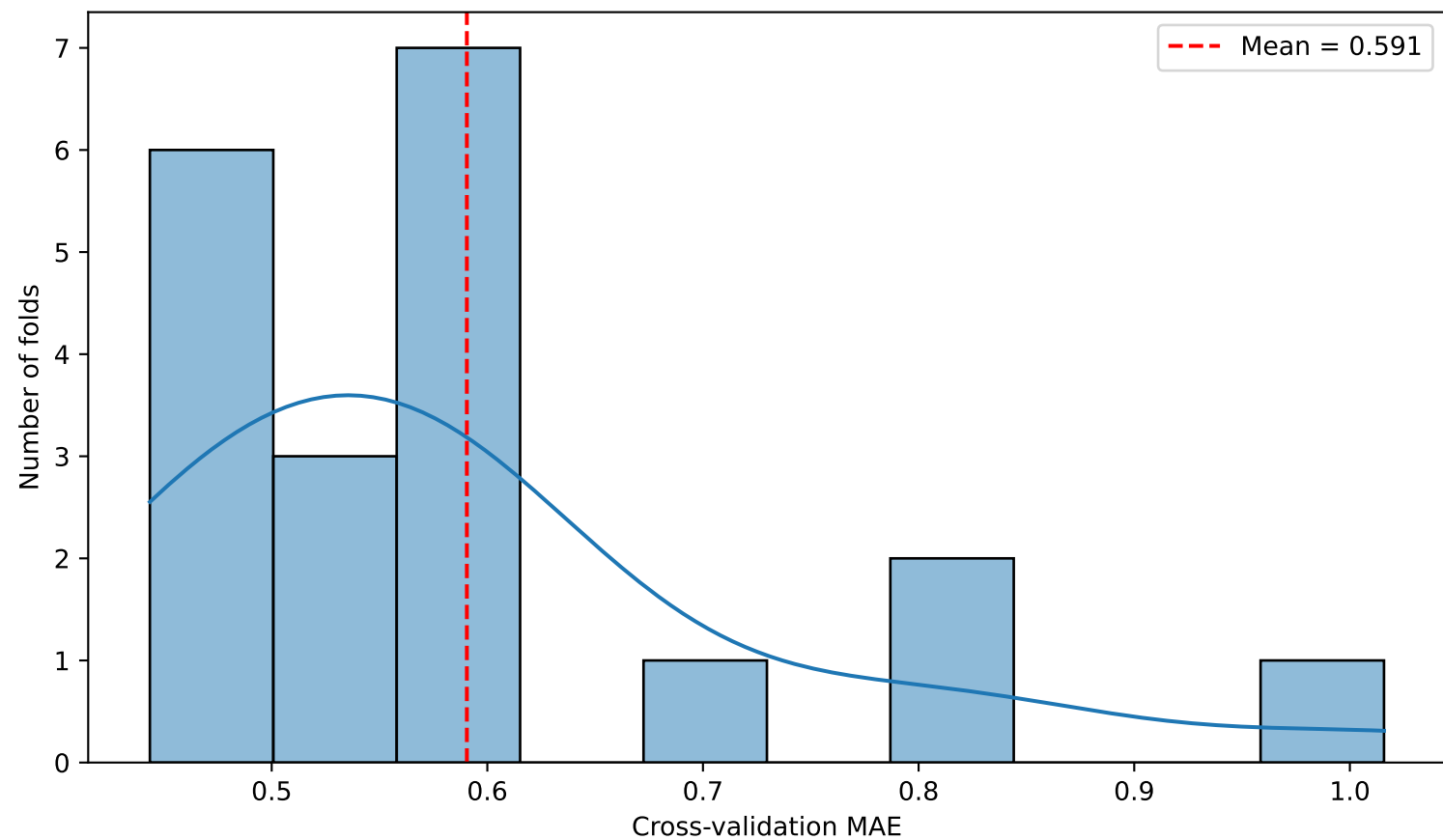
Distribution of MAE Errors in Cross-Validation
