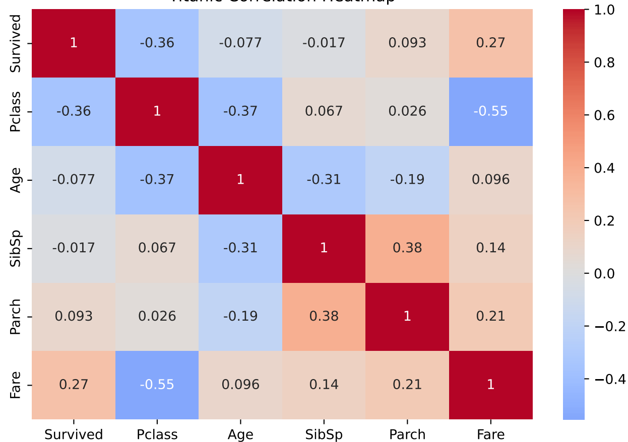
Titanic Correlation Heatmap
