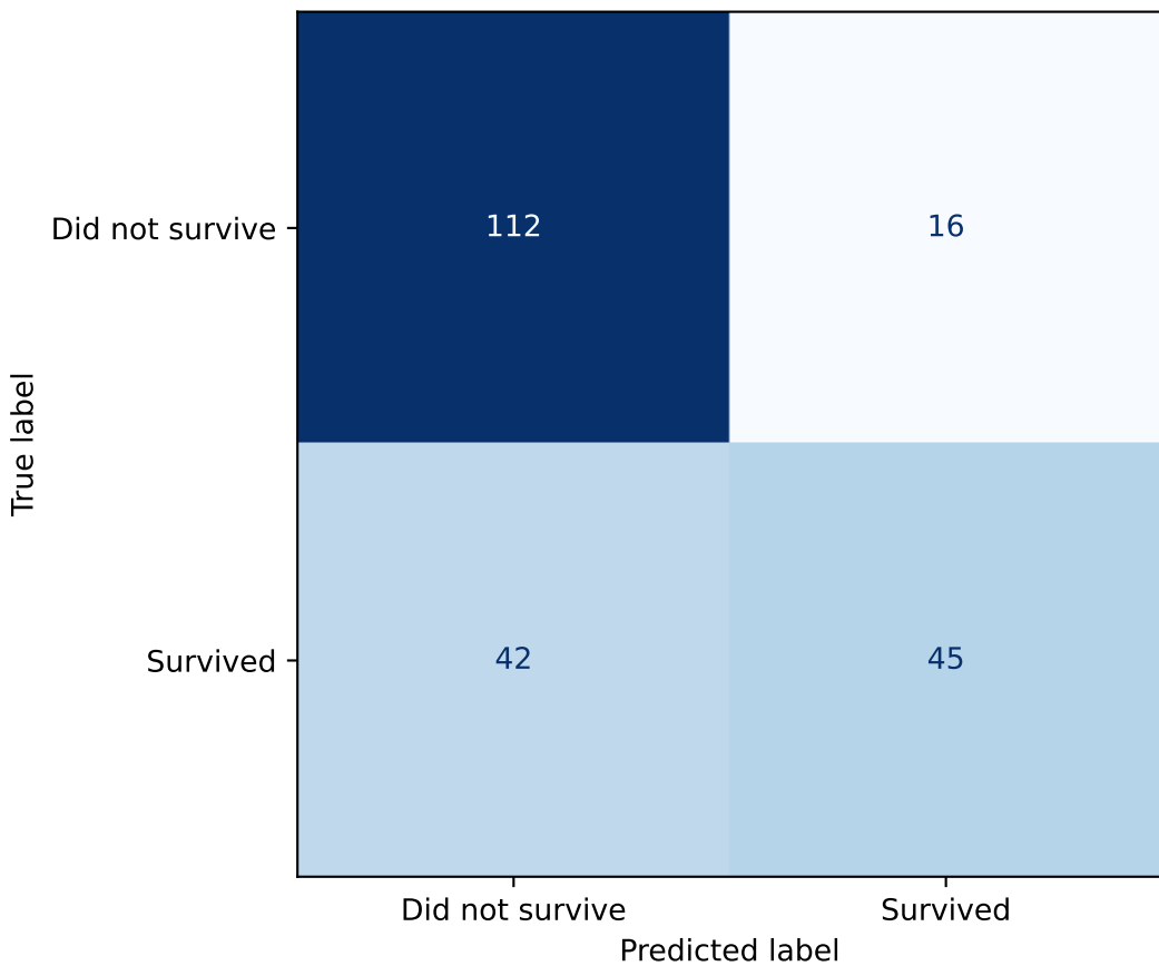
Baseline SVC Confusion Matrix
