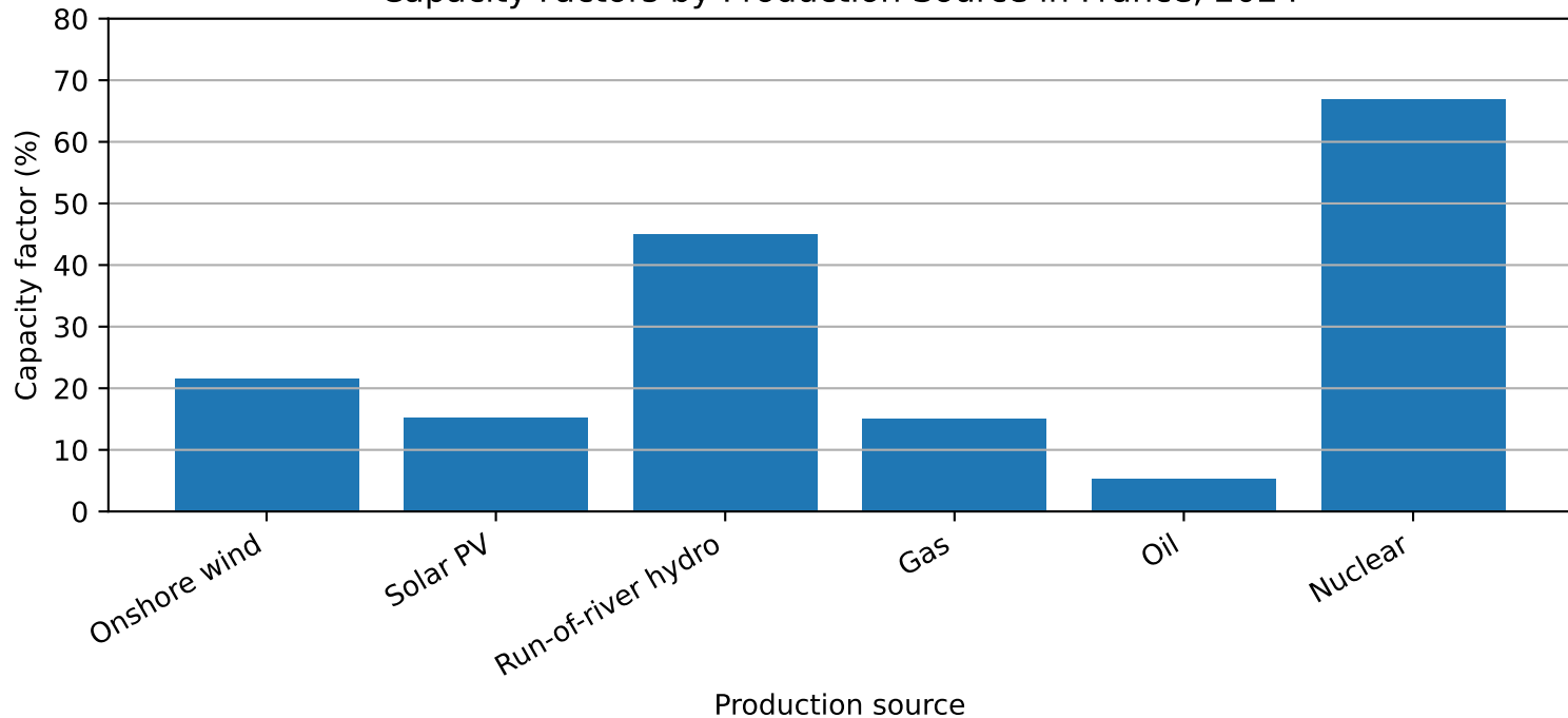
Capacity Factors by Production Source in France, 2024
