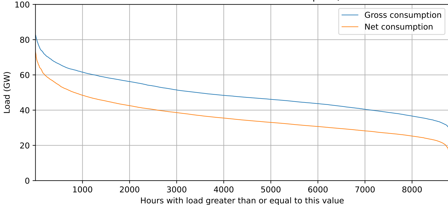
Load Duration Curves of Gross and Net Consumption, France 2024
