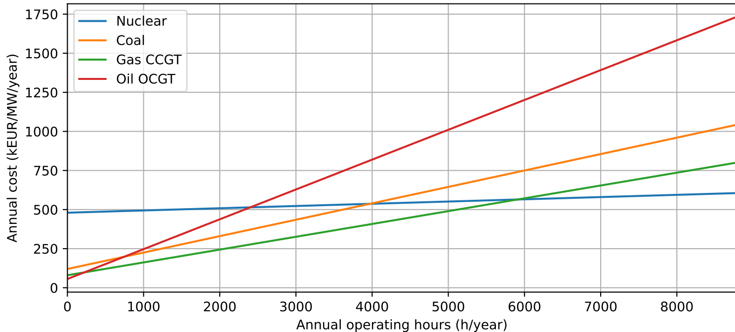
Annual Production Cost for 1 MW of Capacity
