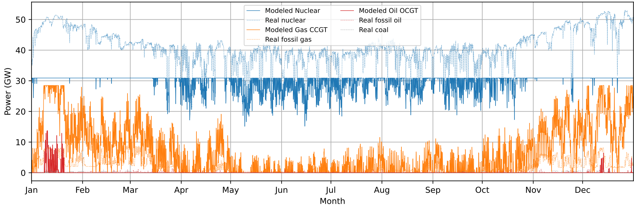
Modeled and Real Dispatchable Production in France, 2024
