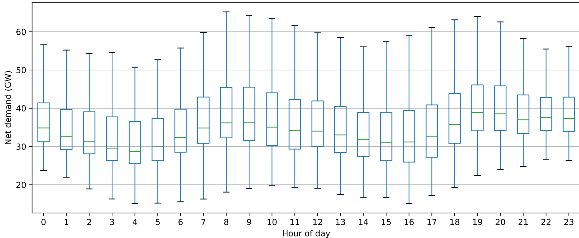
Statistical Distribution of Net Demand by Hour, France 2024
