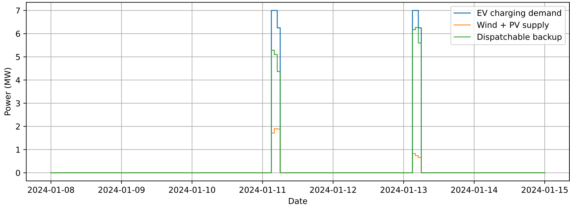
EV Charging Demand and Supply, 8-15 January 2024
