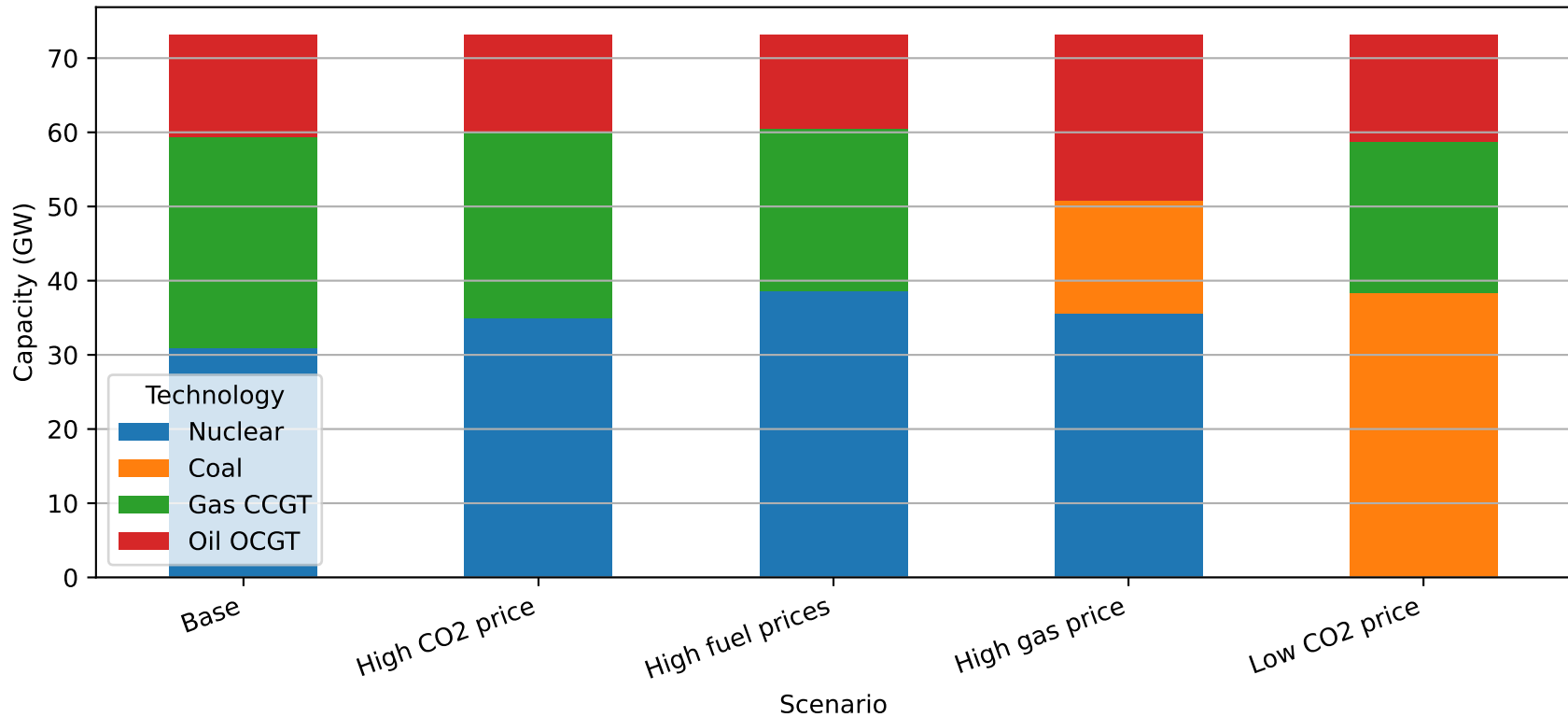
Optimal Dispatchable Capacity Under Fuel and Carbon Price Scenarios
