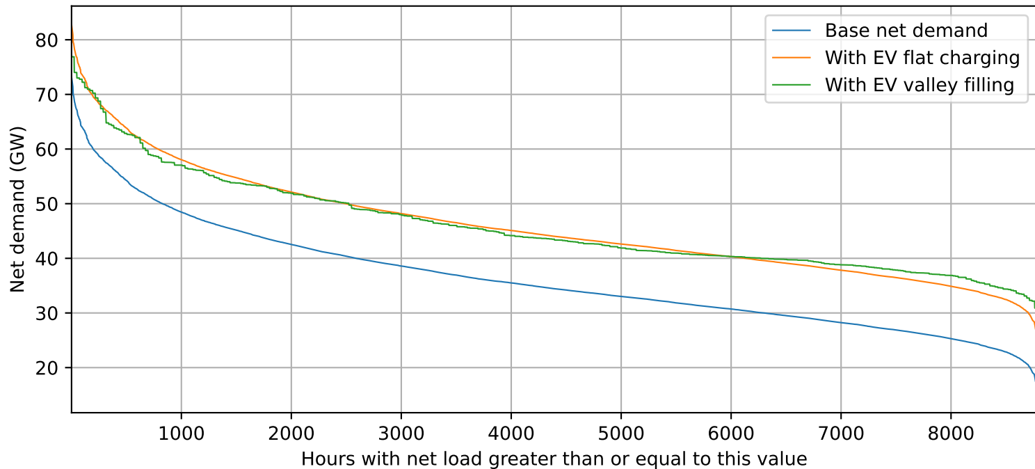
Effect of Electric Vehicle Charging on Net Load Duration Curves
