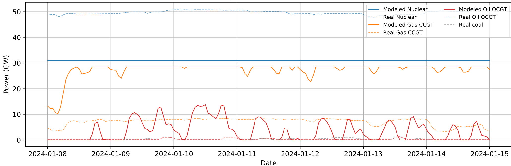
Modeled and Real Dispatchable Production, 8-15 January 2024
