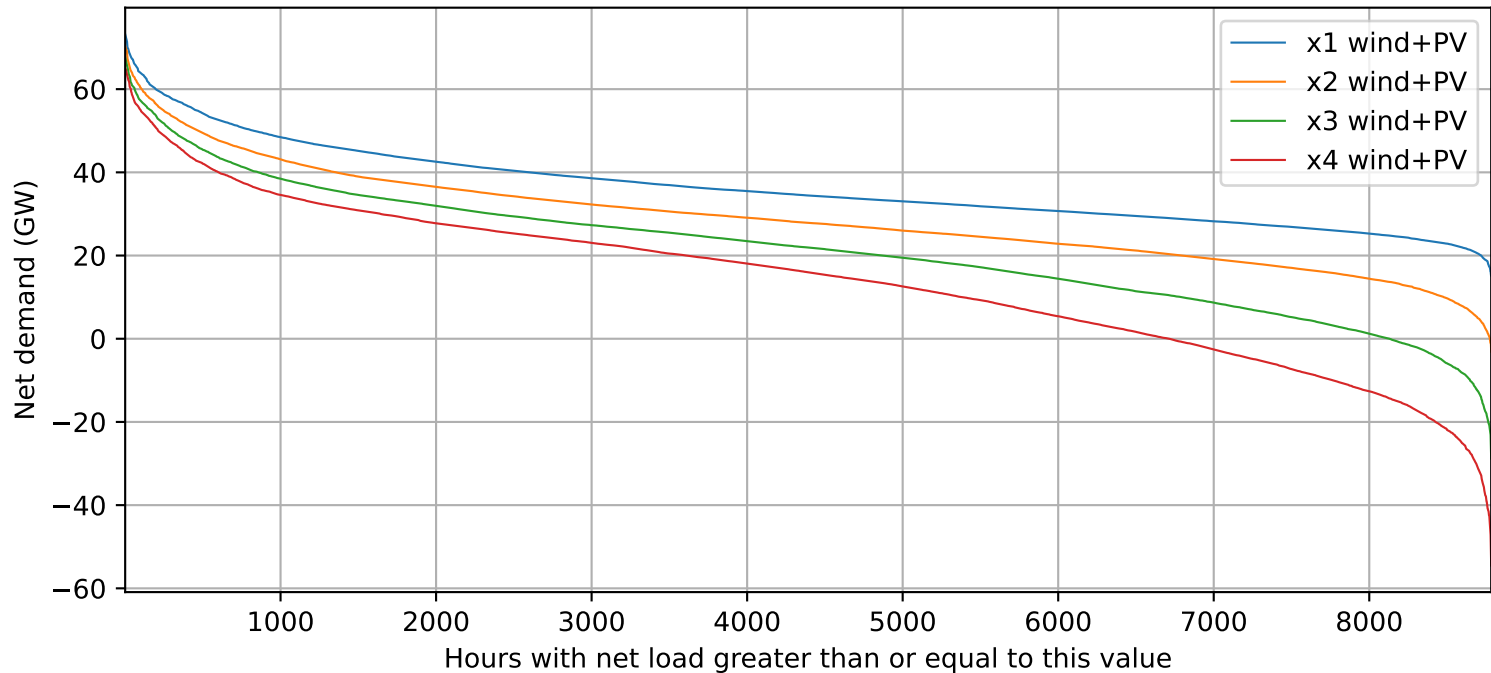
Net Load Duration Curves with Increased Wind and PV
