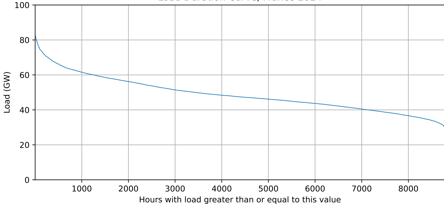
Load Duration Curve, France 2024
