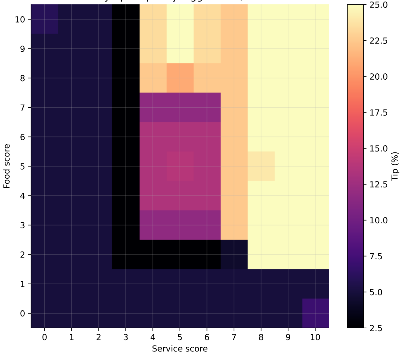
Mean fuzzy tip output by logged food/service case
