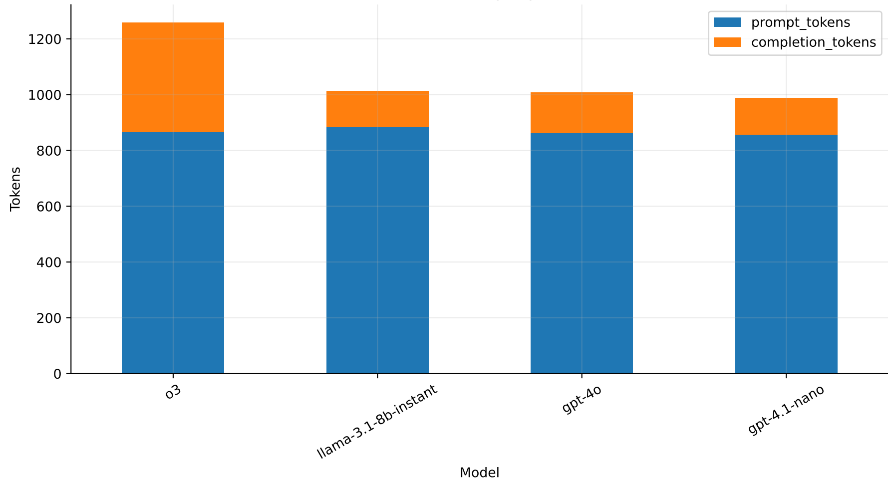
Mean token usage by model
