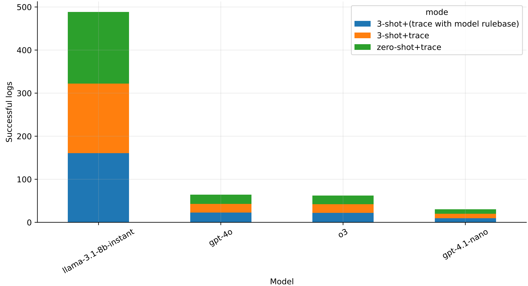
Successful explanations by model and mode
