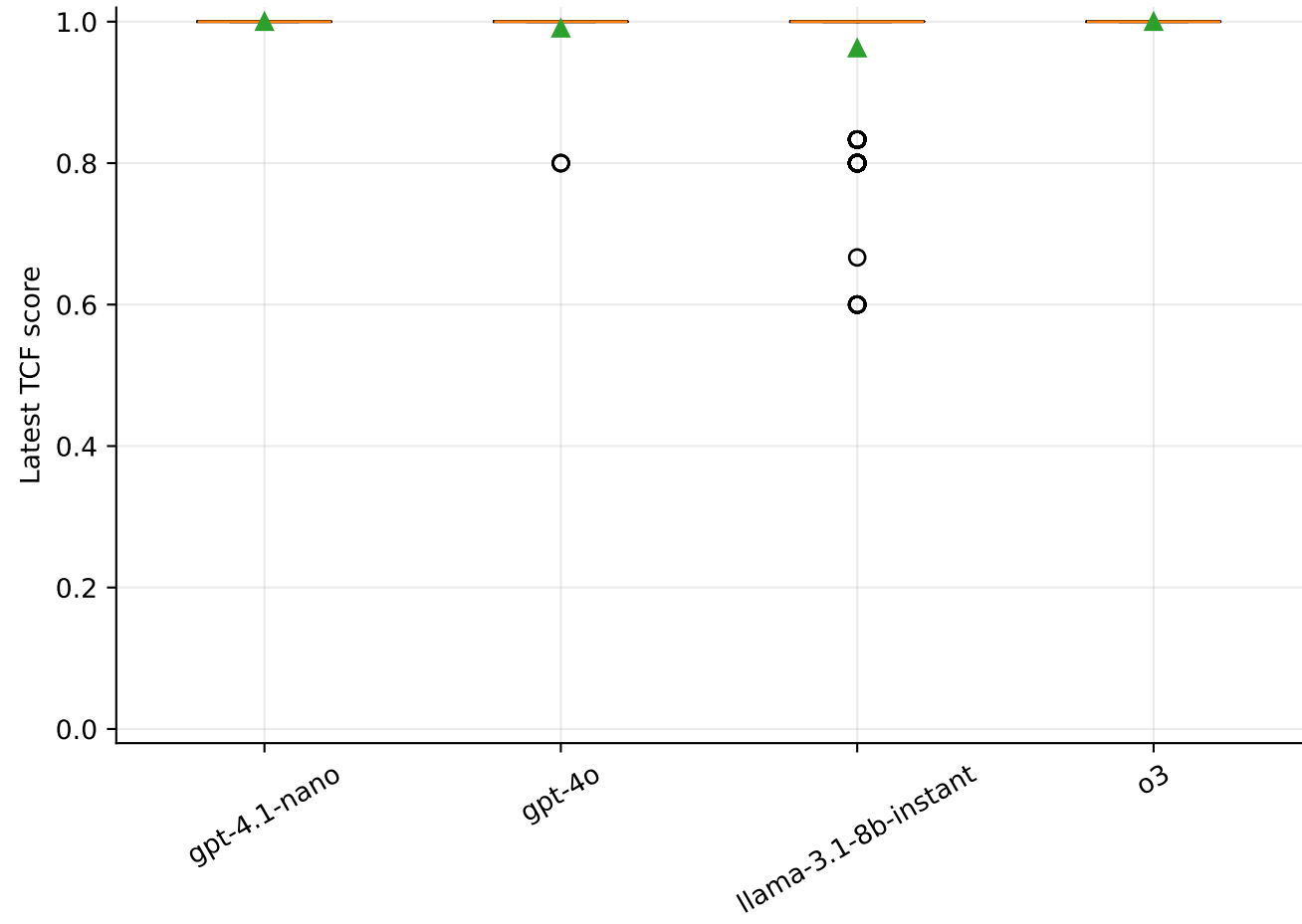
TCF by generation model
