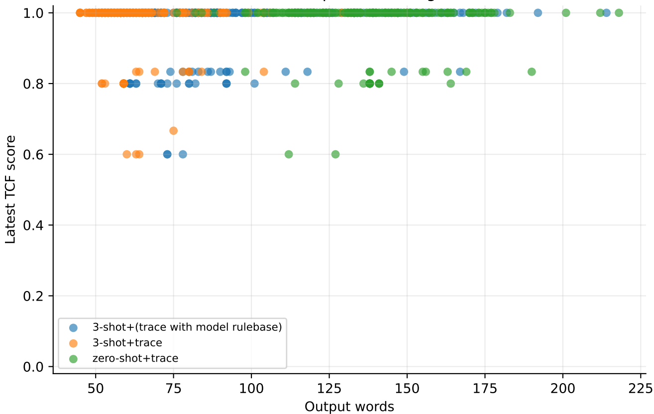
TCF vs explanation length
