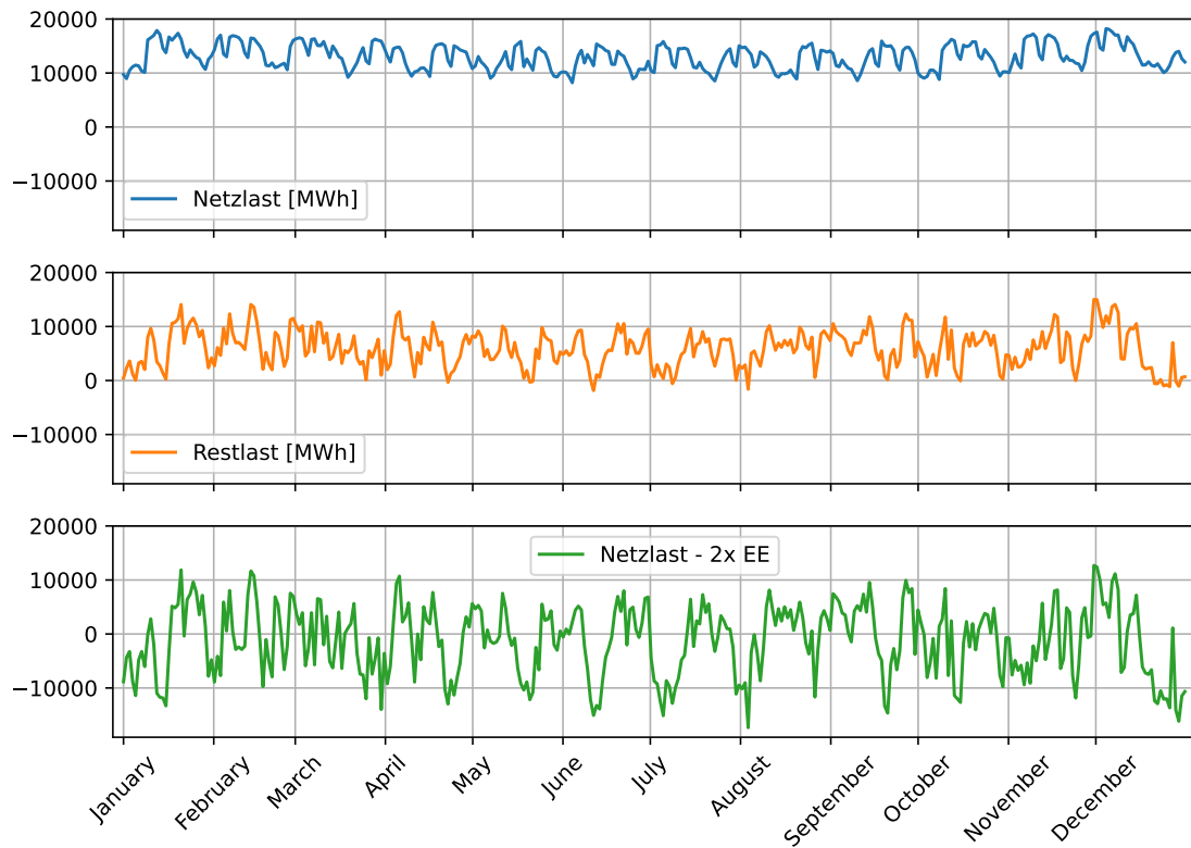
Abbildung 6.2: Example solution doubling Renewable Energy (RE)
