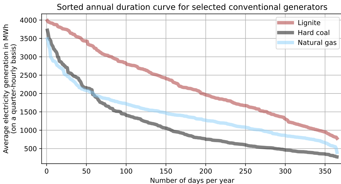
Abbildung 6.7: sorted annual duration curve of selected conventional generators
