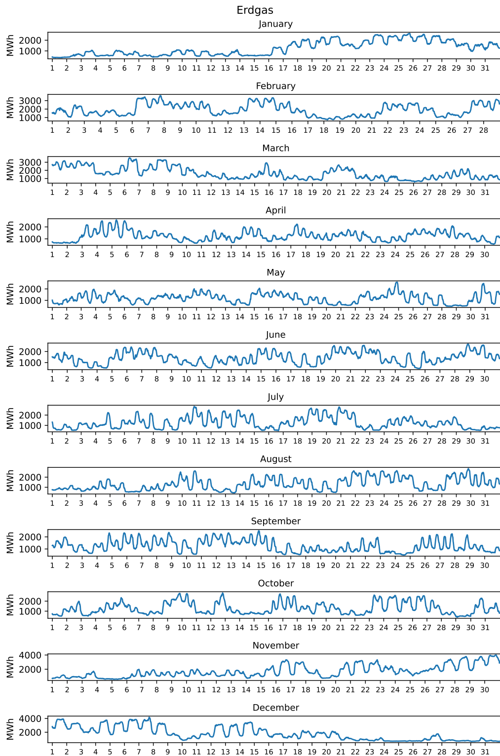
Abbildung 6.6: Annual Profile Natural Gas
