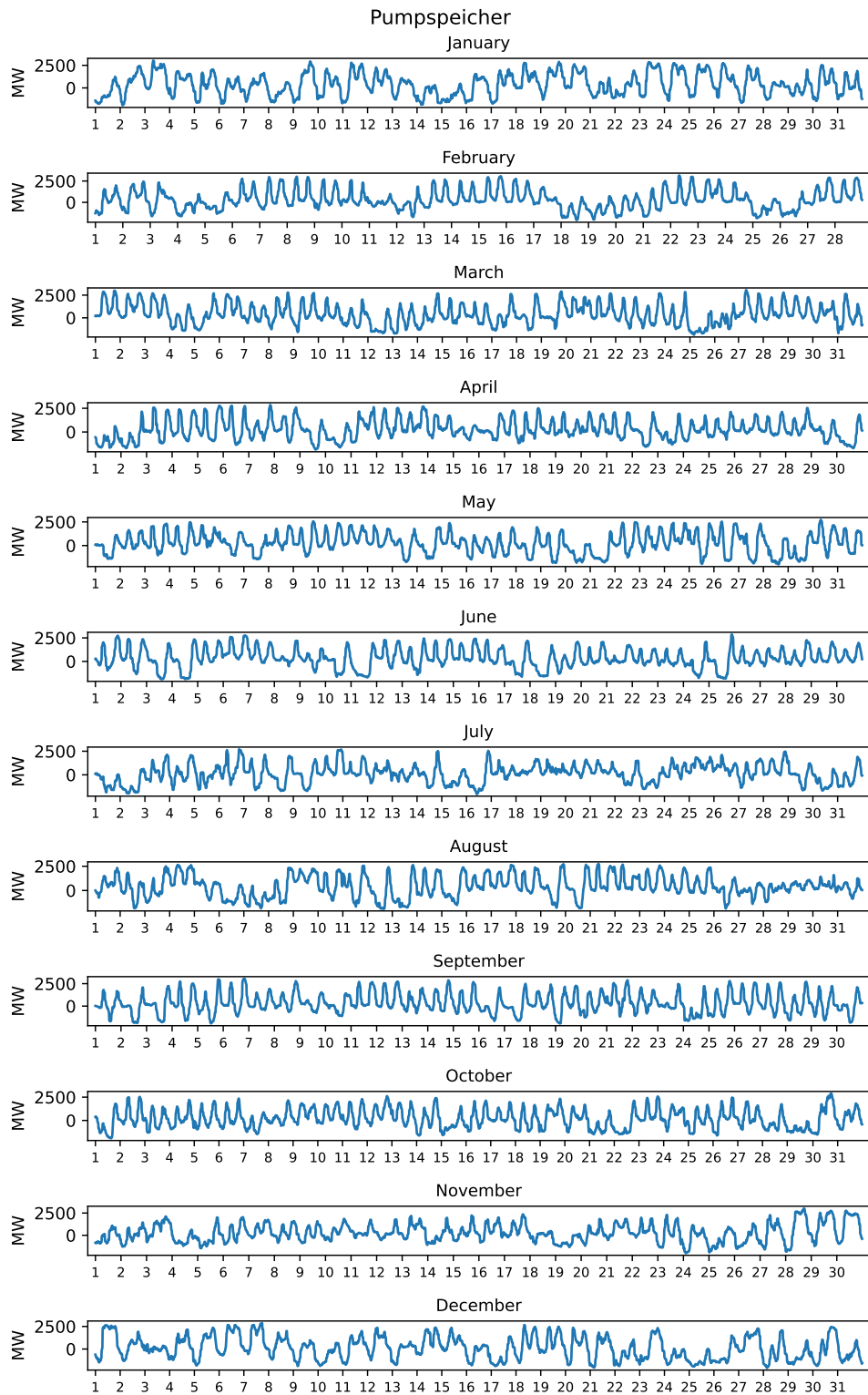
Abbildung 6.15: Annual profile of pumped storage in Austria 2023
