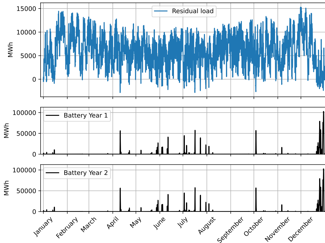
Abbildung 7.3: Residual load 2023 and annual cycle of a storage with charge and discharge efficiency 0.9
