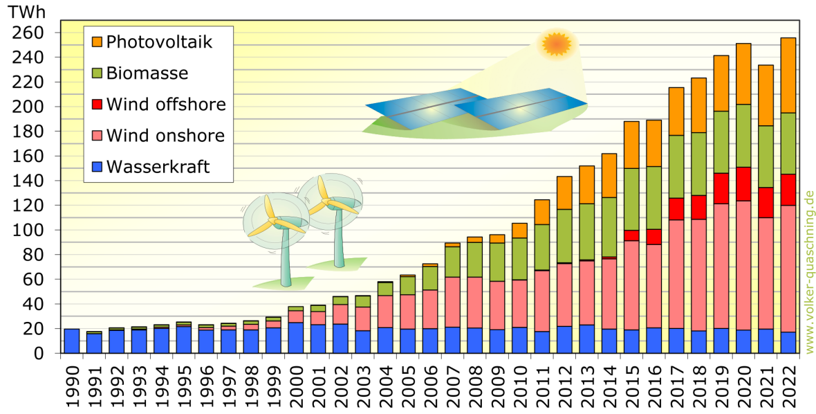
Abbildung 7.1: Renewable electricity generation in Germany since 1990
