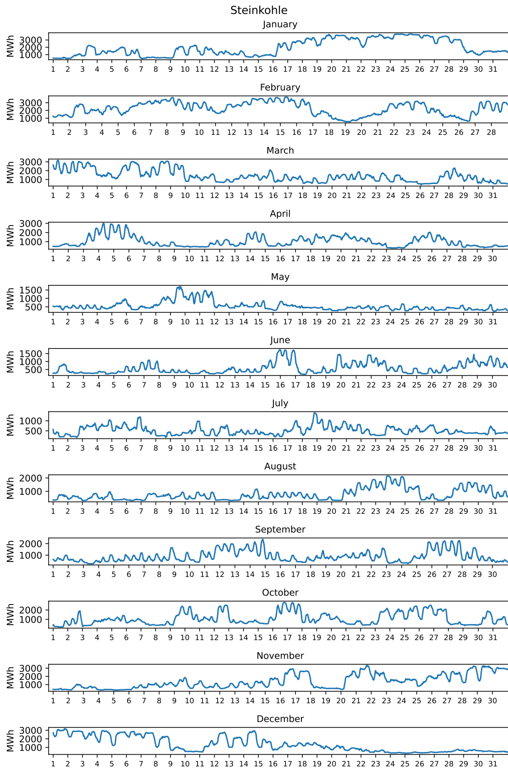
Abbildung 6.5: Annual Profile Hard Coal
