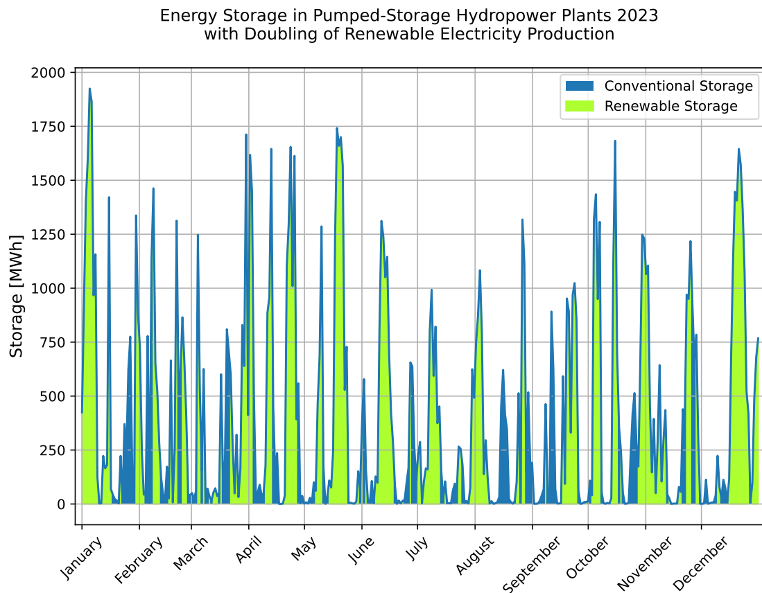
Abbildung 6.12: Energy Storage in Pumped-Storage Hydropower Plants 2023
