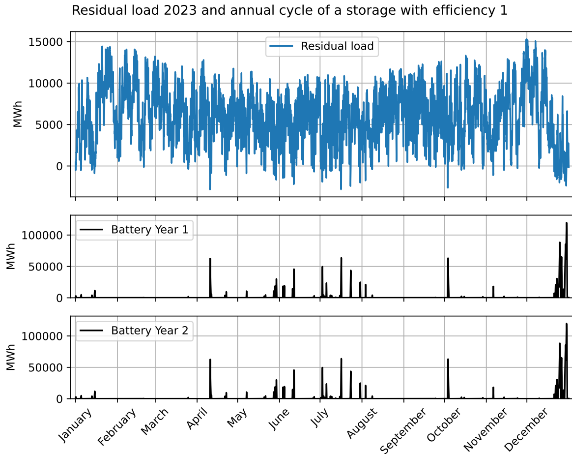
Abbildung 7.2: Residual load 2023 and annual cycle of a storage with efficiency 1
