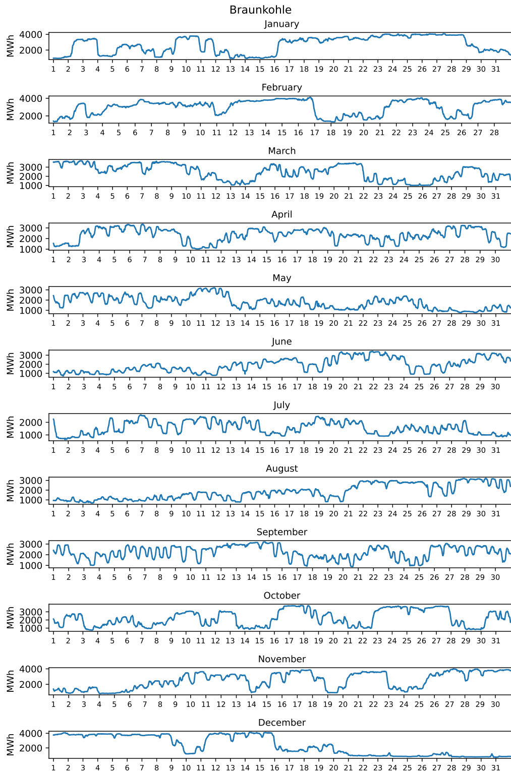
46 Abbildung 6.4: Annual Profile Lignite
