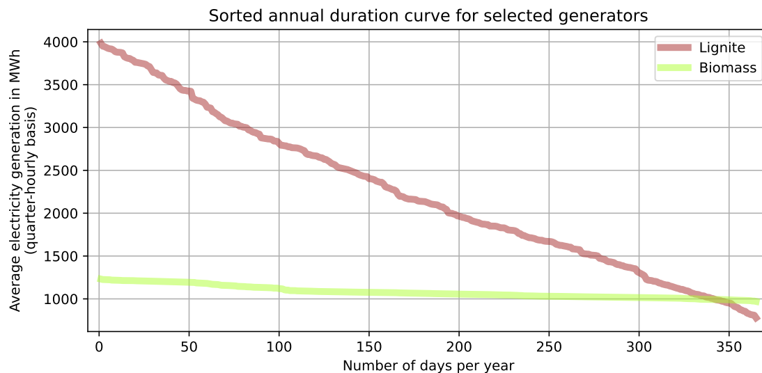
Abbildung 6.10: Sorted annual duration curves for selected generators
