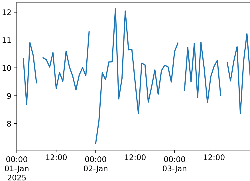
Time Series with Missing Values
