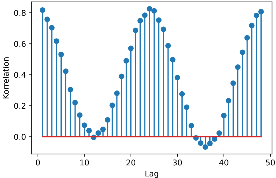
Autokorrelation (NumPy)
