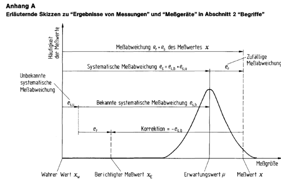
Abbildung 4.1: Measurement result according to DIN 1319
