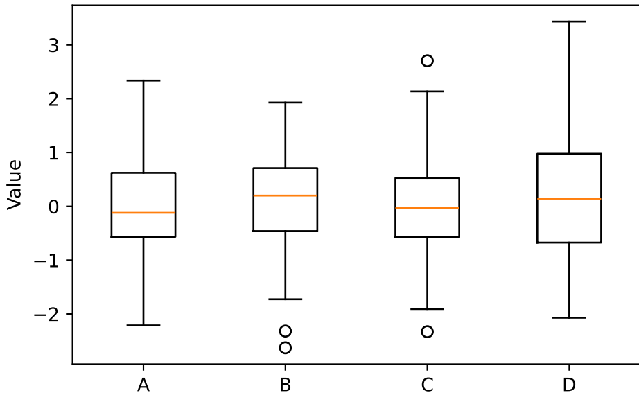
Box Plot
