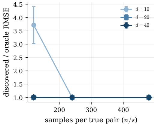
(b) discovery cost
