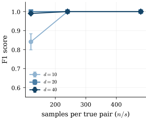
(a) graph recovery
