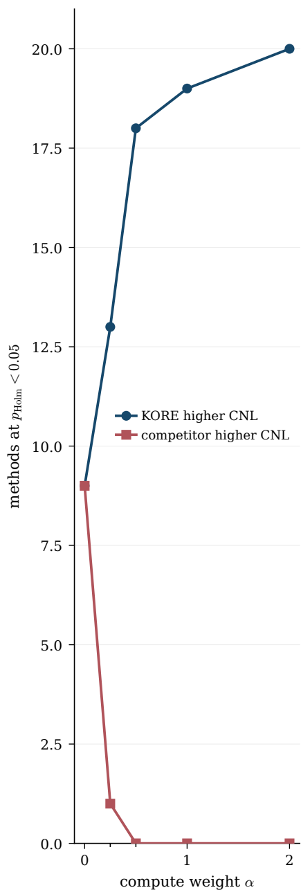
(b) sensitivity to \alpha
