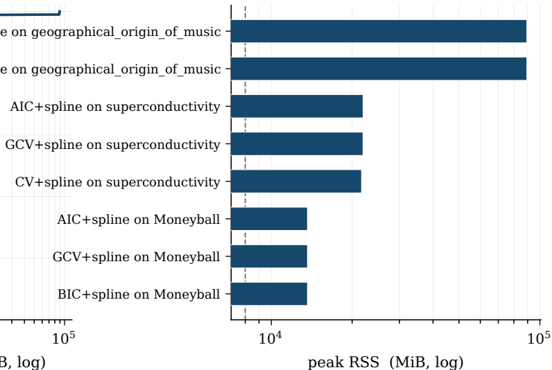
(b) top RSS offenders
