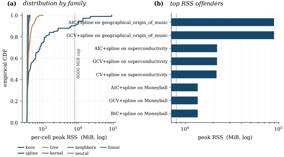
Figure 26. Per-cell peak resident-set size on the real-world benchmark. Panel (a): empirical CDF of cell peak RSS aggregated by method family, with the soft per-cell cap drawn as a vertical reference. Panel (b): the top (method, dataset) RSS offenders.
