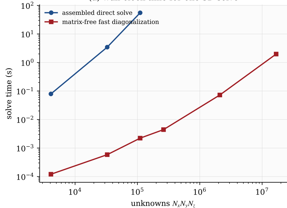
(a) wall-clock time for one 3D solve
