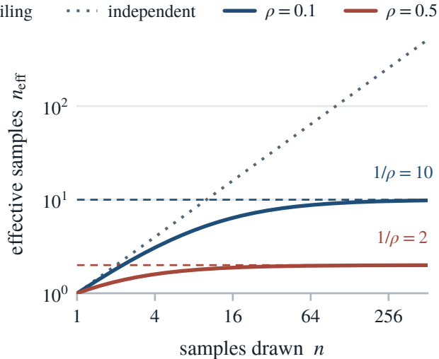
(b) Estimation hits the correlation ceiling
