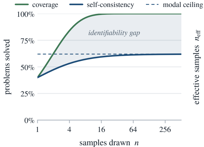
(a) Selection hits the modal ceiling
