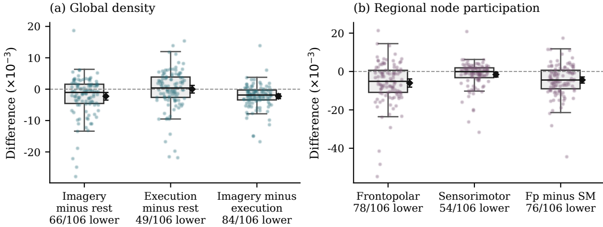
Figure 2. Participant-level RSEC differences ( n = 106 ). (a) Global density contrasts. (b) Imagery–rest node participation over frontopolar (Fp: Fp1/Fp2/Fp2) and sensorimotor (SM: C3/Cz/C4) electrodes and their regional difference. Points are participants; boxes show median and interquartile range with 1.5-IQR whiskers. Diamonds and bars show means and 95% participant-bootstrap intervals. Labels count negative differences.
