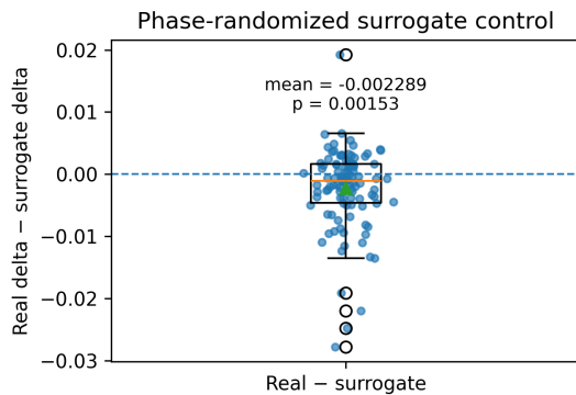
Figure 3. Phase-randomized surrogate control. Each point is one participant's real imagery–rest change minus the surrogate change ( n = 106 ). The green triangle marks the mean; the box shows the median and interquartile range, with 1.5-IQR whiskers. Open circles are boxplot outlier markers for participants also shown by filled points. The displayed p = 0.00153 is unadjusted; the four-test Holm value is 0.00444. Negative values indicate a more negative real effect.
