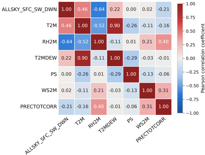
Rize: correlation matrix (target > 0)
