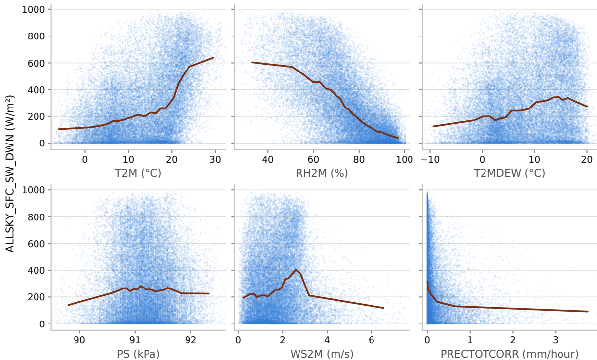
Size: meteorological variables against irradiance (hours with target > 0; line: binned median)
