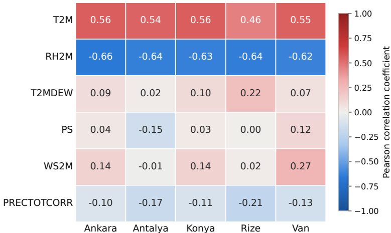
Correlation of each variable with irradiance (hours with target > 0)
