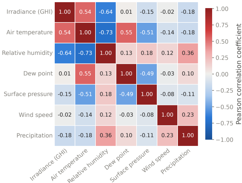
Antalya: correlation matrix (daylight)
