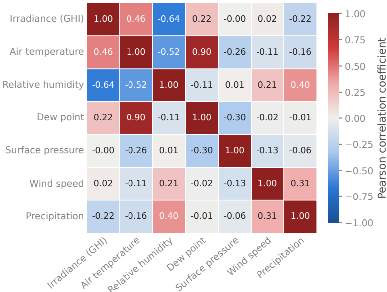
Rize: correlation matrix (daylight)
