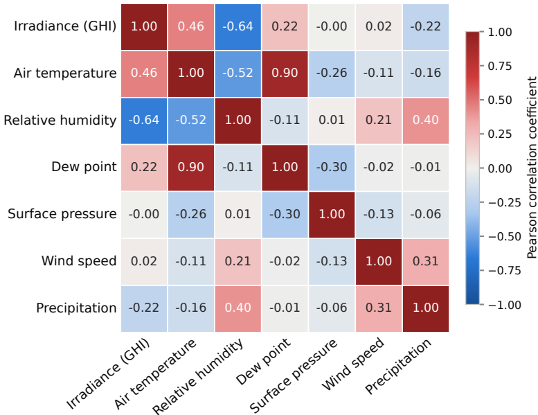
Size: correlation matrix (daylight)
