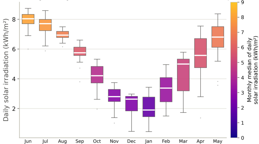
Antalya: daily solar irradiation over the last 12 months (Jun 2025 - May 2026)
